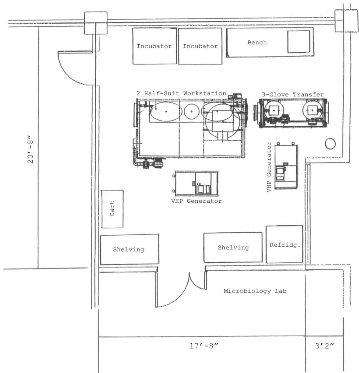
Scale: 1"=5' Small Room Layout
